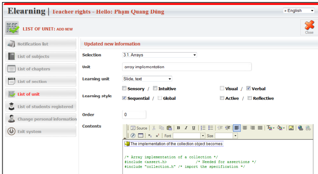
Figure 3. A screen shot from POLCA to which a teacher adds a learning object
