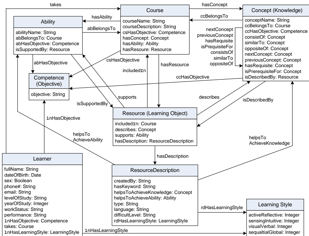
Figure 1. General layout of the domain ontology
